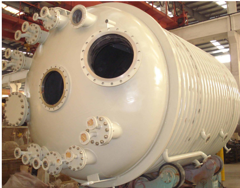
带搅拌的配料罐 With Stir Ingredients Tank Material: 00Cr19Ni10 (304L) Size: DN2800×16 L=5400
