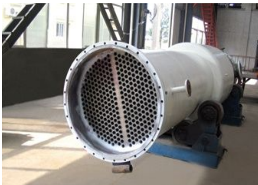
氯化钙浓缩塔 Chlorate Calcium Concentrator
