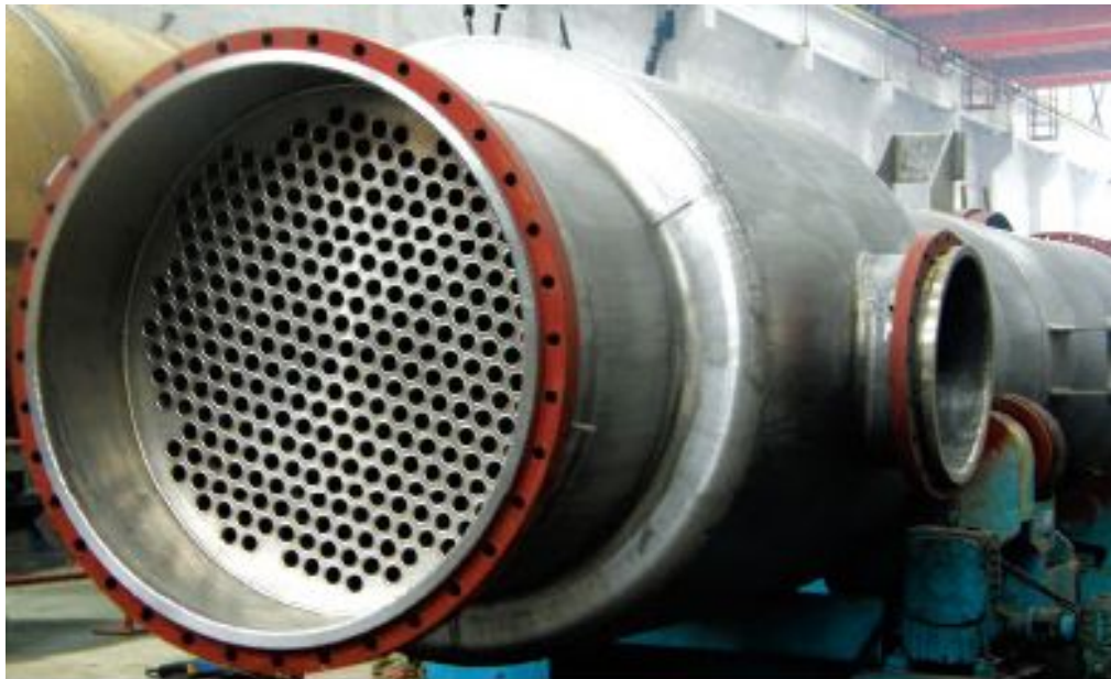
V效加热室 Heating Chamber
